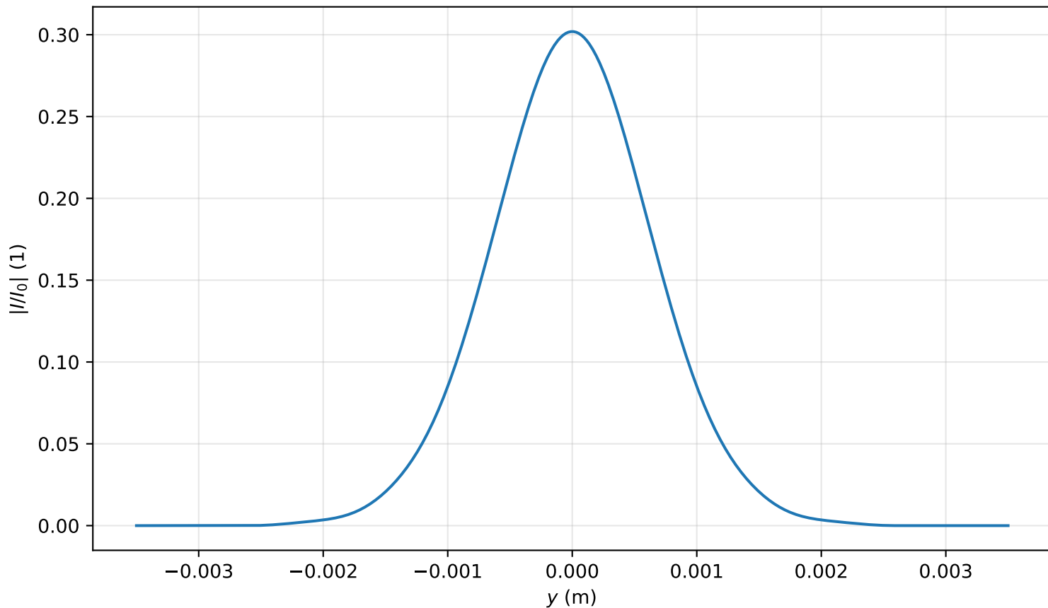
Intensity profile I(x=0, y, z=3.821)/I_0 , P_{in}=0.3P_{cr} , artificial time
